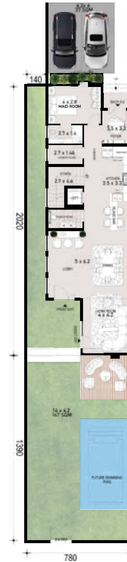
G FLOOR PLAN
